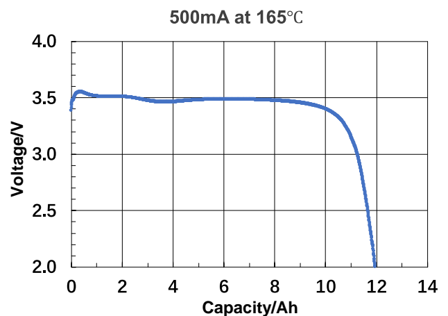
Discharge curve
