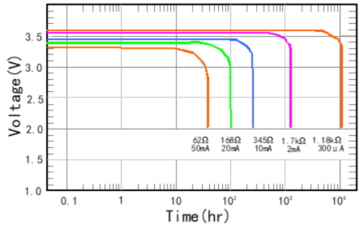
Capacity VS. Current
